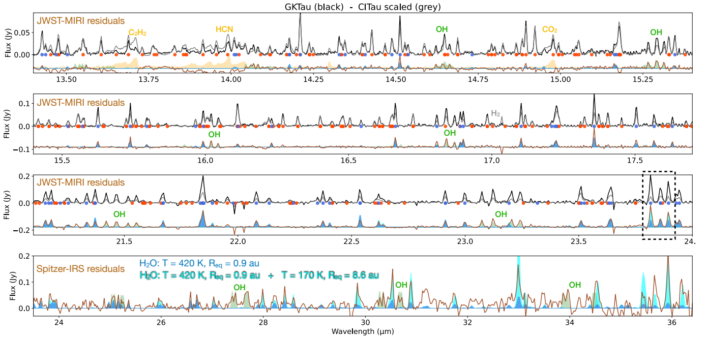
Figure 10. Broader view of excess cool component in rotational water emission in GK Tau, using CI Tau as template for the hot component as in Figure 4. The same scaling and subtraction procedure described in Section 3 is applied here, where residuals after subtraction are shown in brown for MIRI (top 3 panels) and IRS (bottom panel). A two temperature fit is shown in blue (only the T \approx 400 K component) and cyan ( T \approx 400 K and T \approx 170 K components together), with best-fit values as reported in Appendix B. The dashed box marks the two MIRI lines discussed in the text. Other molecules are reported and labelled in different colors for reference.
