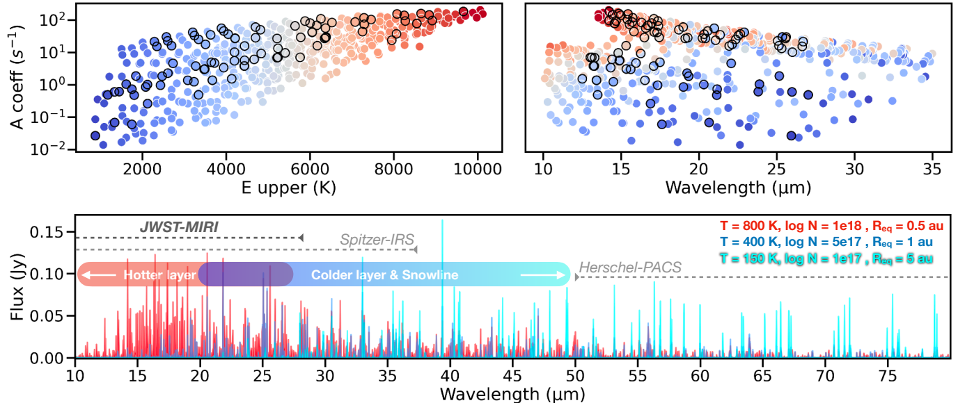
Figure 1. The distribution of upper level energies E_u and Einstein- A coefficients (top plots, with color-coding reflecting E_u values) across infrared wavelengths naturally traces radial temperature gradients in inner disks within and across the water snowline (bottom plot, where the spectrum is scaled to a distance of 130 pc). Partly adapted from Figure 1 in Blevins et al. (2016) and Figure 13 in Banzatti et al. (2023). The MIRI lines used in the analysis in Section 3 are marked with black circles.
