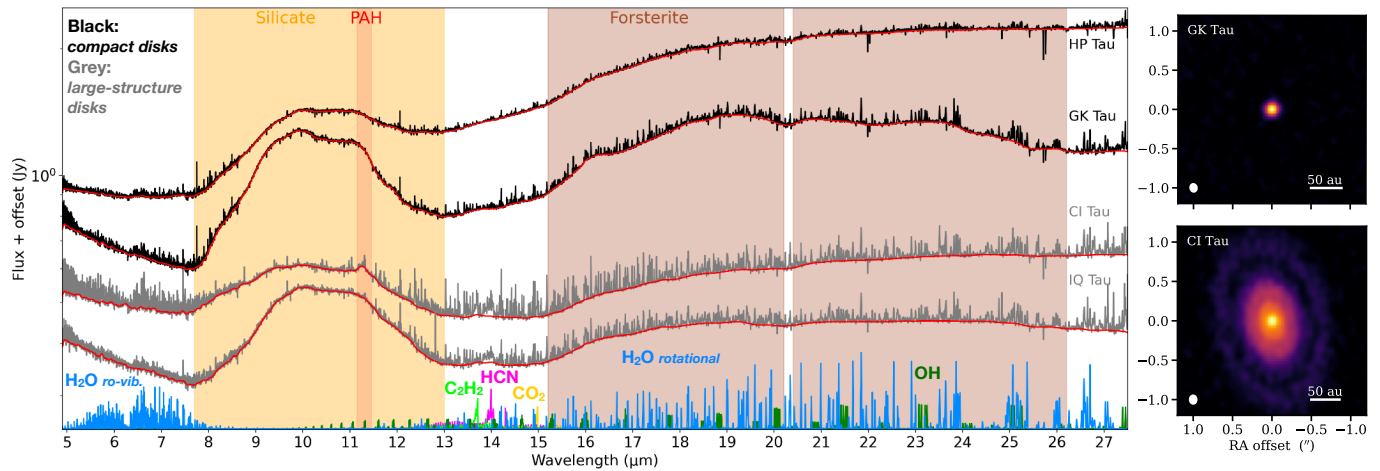
Figure 2. JWST MIRI-MRS spectra for the four disks. For clarity, the spectra are offset vertically by the following additive shifts: 0.05 Jy in CI Tau, 0.17 Jy in GK Tau, 0.4 Jy in HP Tau. Illustrative models of molecular emission are shown for guidance at the bottom. Prominent dust features are approximately identified and marked with shaded regions. The estimated continuum that is subtracted before analyzing the water spectra is shown in red on each spectrum. Two ALMA images are shown to the right for reference of disk sizes and structures (the whole sample is included in Appendix A).
