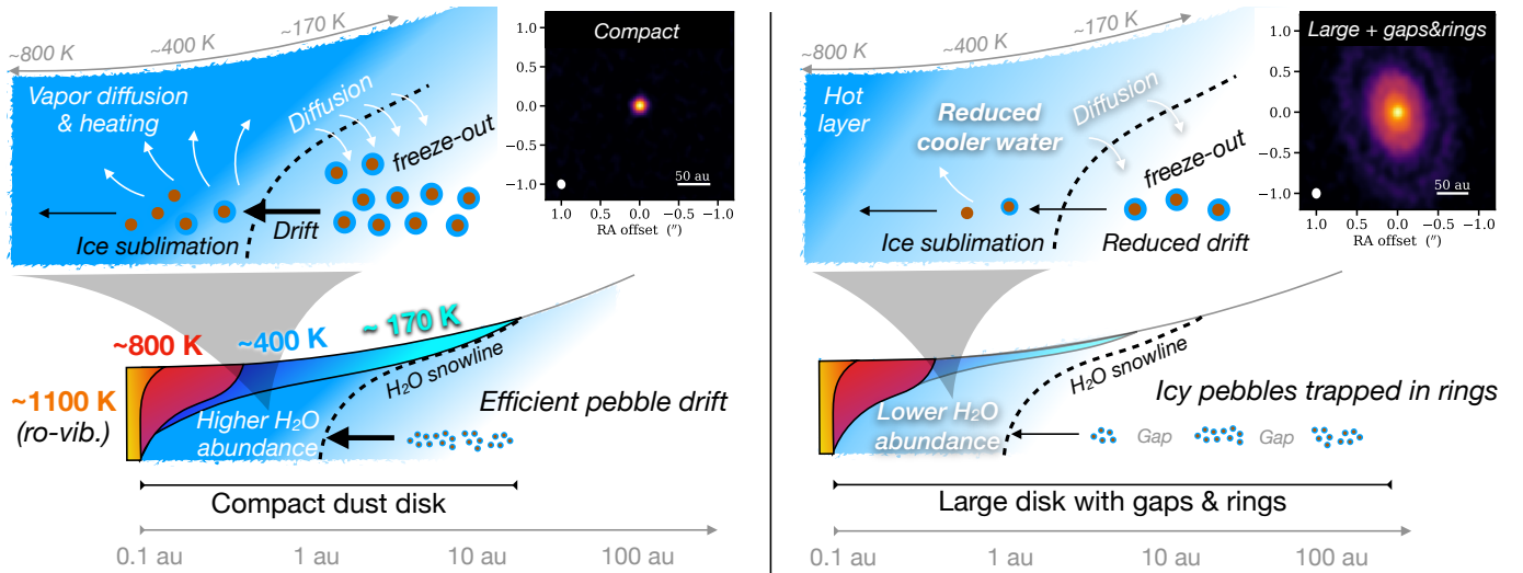
Figure 7. Illustration of the interpretation of the results in the context of the long-established paradigm of inner water enrichment by pebble drift (Cyr et al. 1998; Ciesla & Cuzzi 2006). The insets show the main processes of pebble drift, ice sublimation, and vapor diffusion as included in recent model explorations by Kalyaan et al. (2021, 2023) in the context of how ice delivery and inner disk water enrichment may be regulated by dust gaps observed with ALMA.
