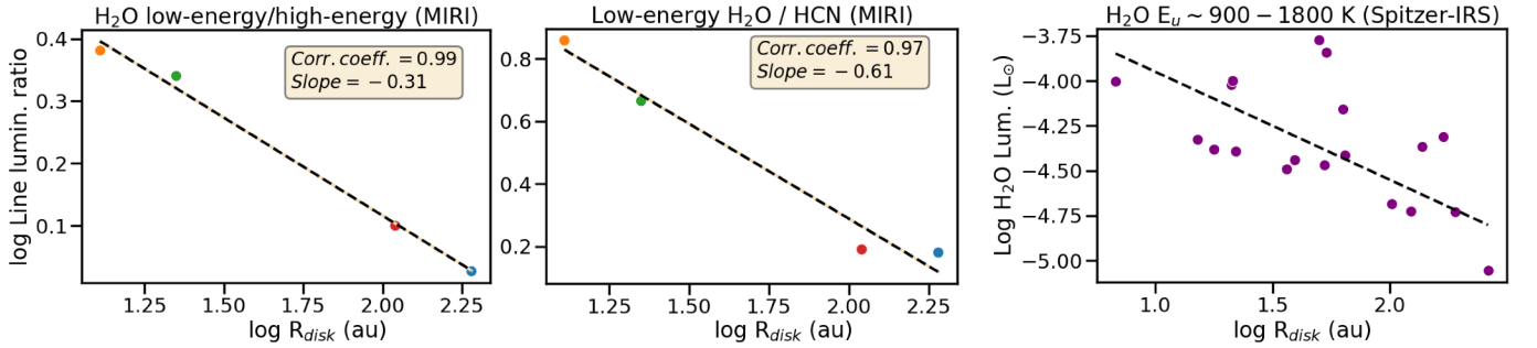
Figure 6. Correlations with dust disk radius R_{\text{disk}} for the luminosity ratio between resolved water low-energy and high-energy lines in MIRI (left), resolved water low-energy lines and the 14\ \mu\text{m} HCN band in MIRI (center), and blended water low-energy lines in Spitzer near 30\ \mu\text{m} (taken from Figure 9 in Banzatti et al. 2023, excluding disks with large inner dust cavities).
